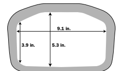
Dimensions transparent sleeve
